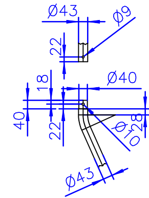
Detail "Y"
