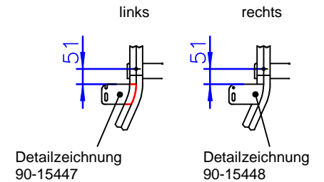
Detail "Y"
